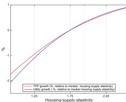
Figure J.5: TFP and indirect welfare effects of increasing housing-supply elasticity.
