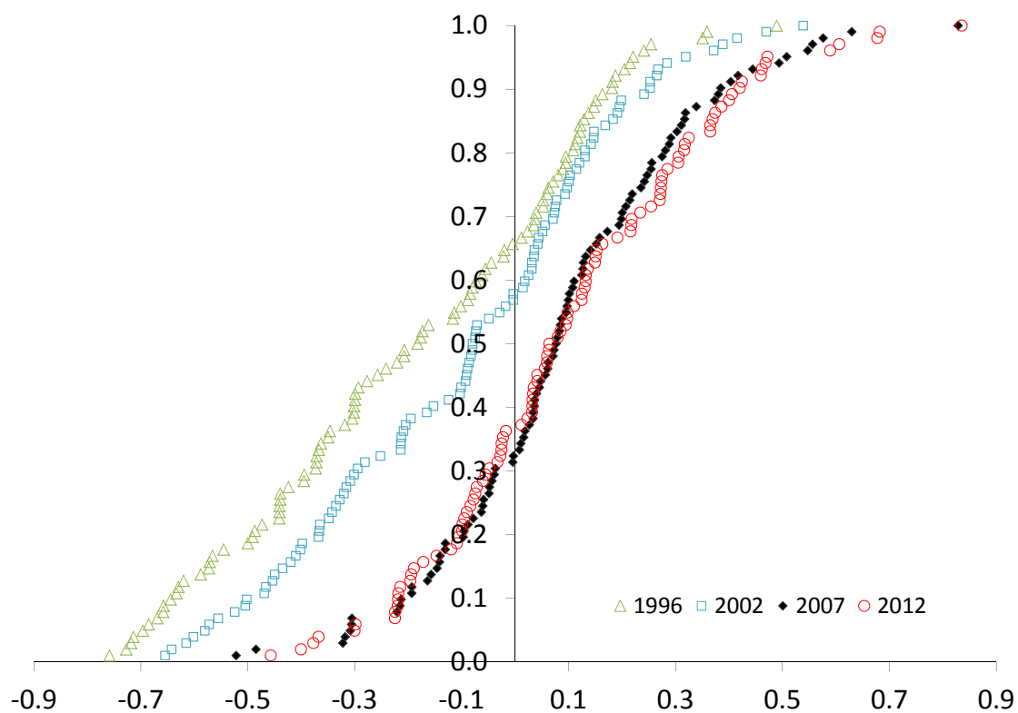
Figure 1: FXAGG distributions
