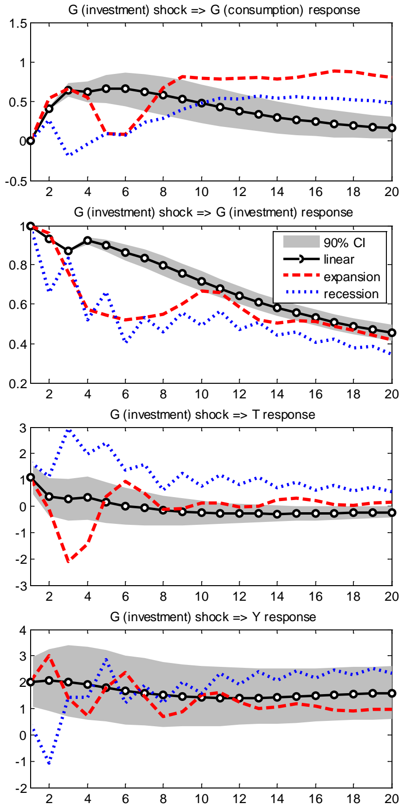
Figure A8. Investment spending: linear model
