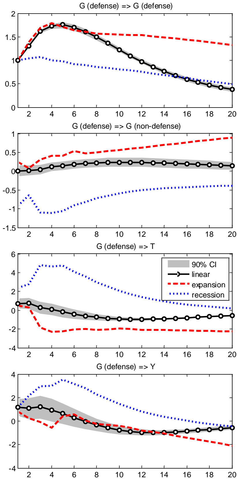
Figure A1. Defense spending: linear model
